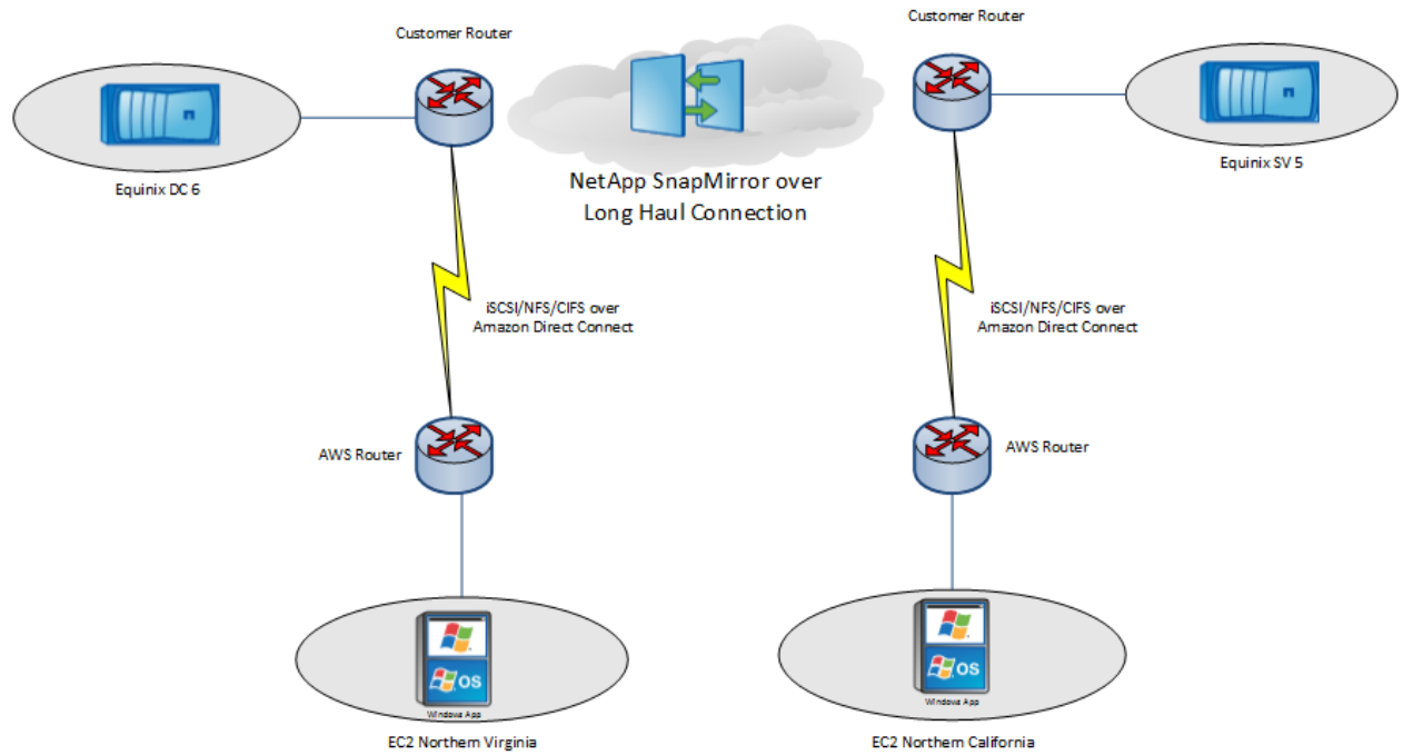
Figure 2) Example of complex routing configuration, including routing over private network between EC2 regions to support SnapMirror replication between colocated data centers (BGP and OSPF).
